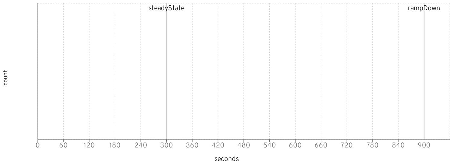
supplierWorker queue
